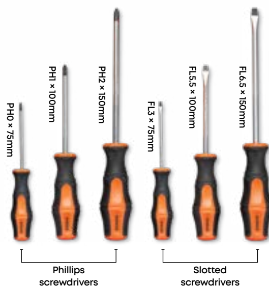
SCDR/R/6/ST
